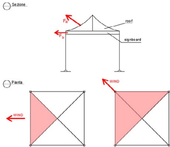
Figure 1 Force application
